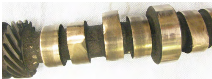
The result of running a flat tappet camshaft using an oil without sufficient ZDDP
