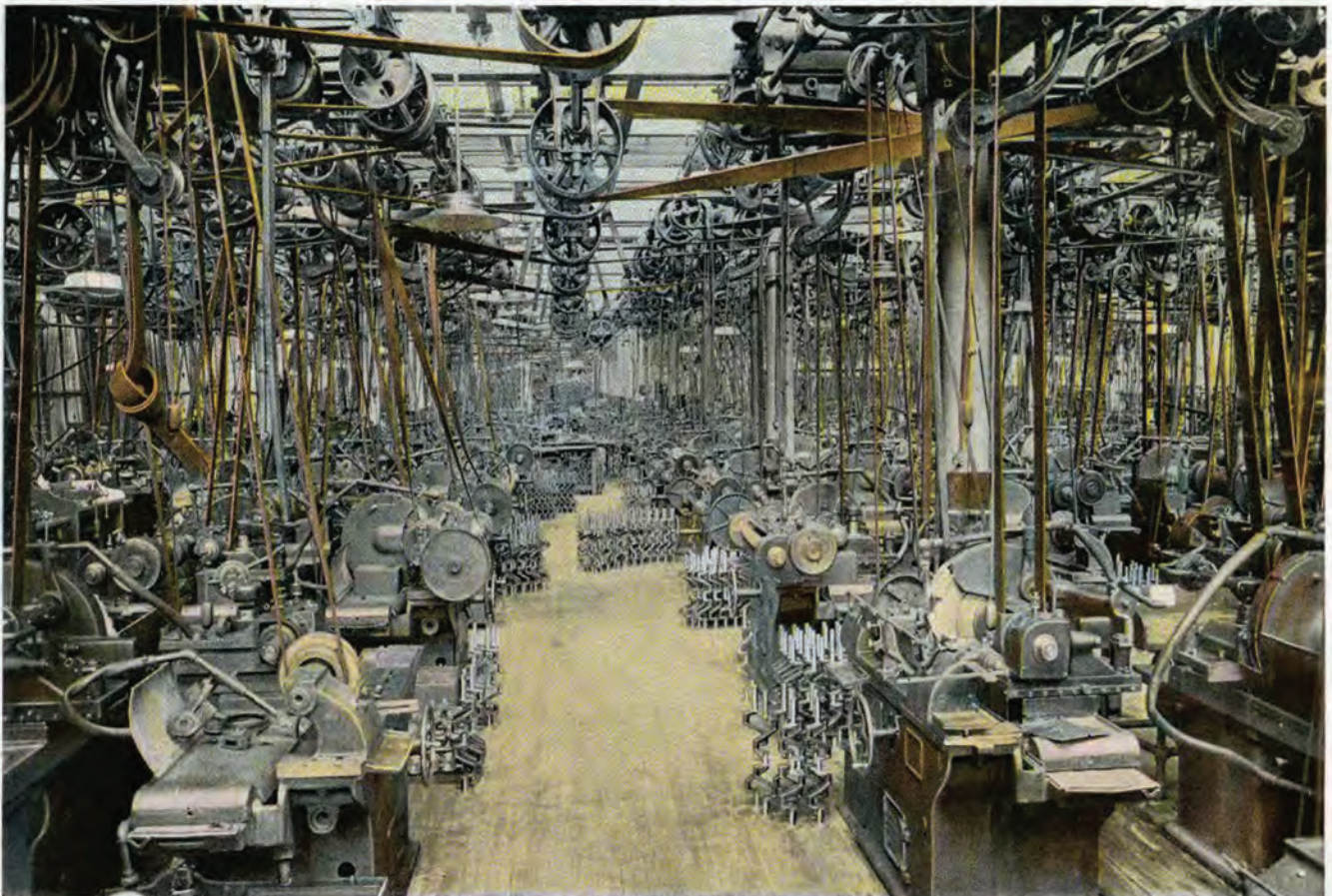
CRANKSHAFT GRINDING DEPARTMENT. 50 MILES OF BELTING ARE USED TO DRIVE FORD MACHINERY.
