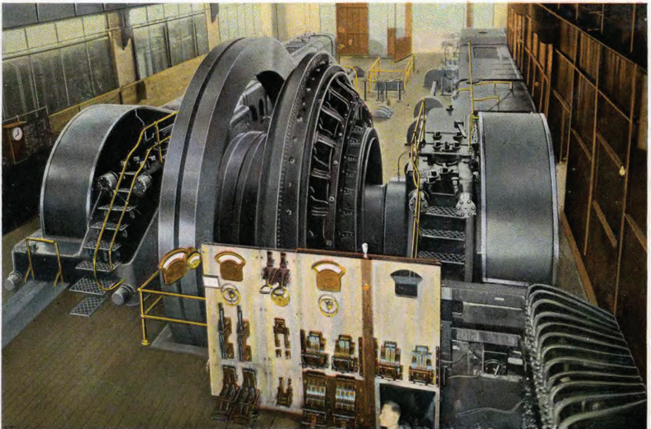
A 6,000 HORSE POWER GAS-STEAM ENGINE. THERE ARE SEVEN OF THESE AT FORD'S.
