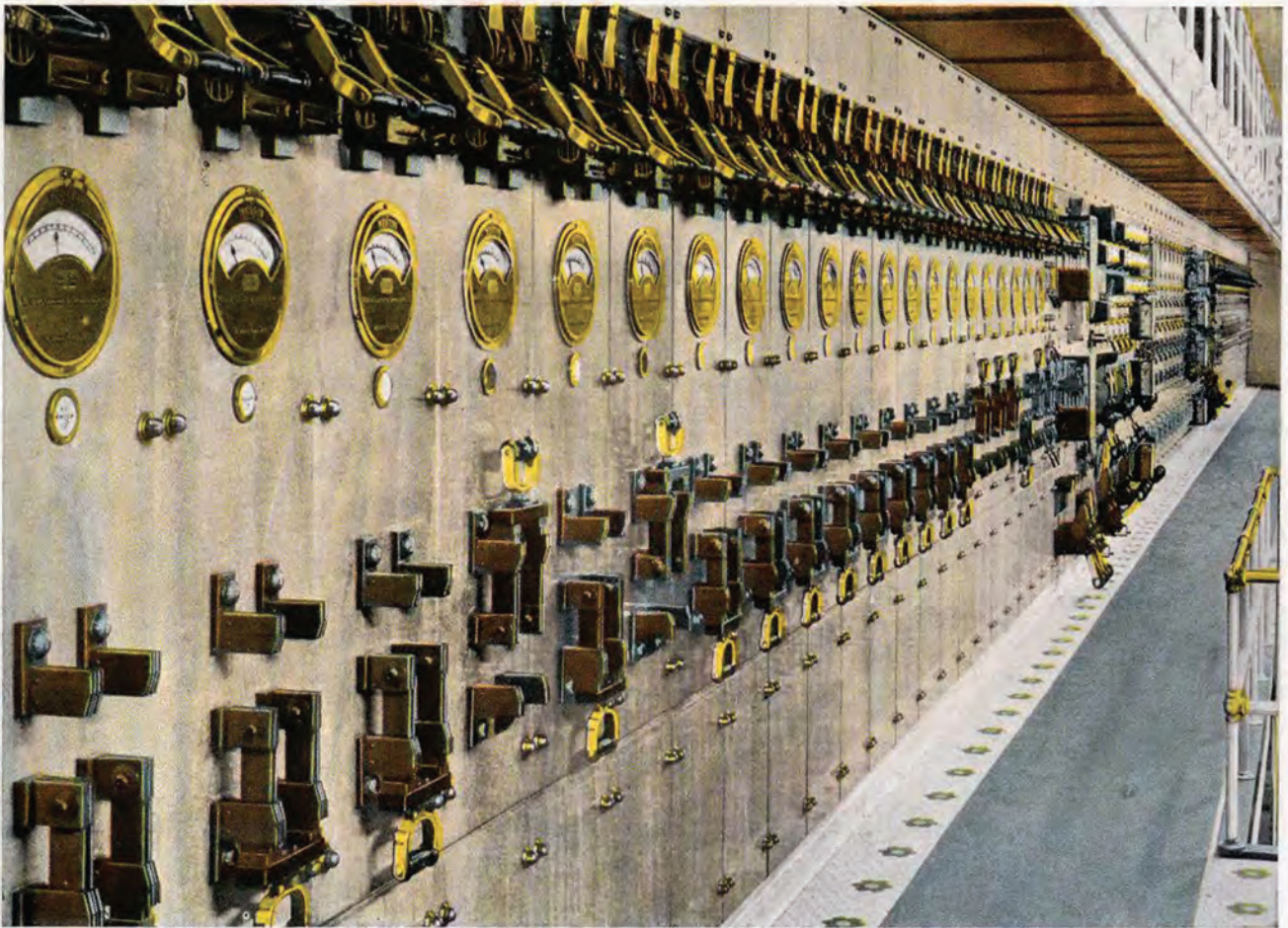
THE LARGEST DIRECT CURRENT CONTROL BOARD IN THE WORLD IN THE FORD POWER HOUSE.
